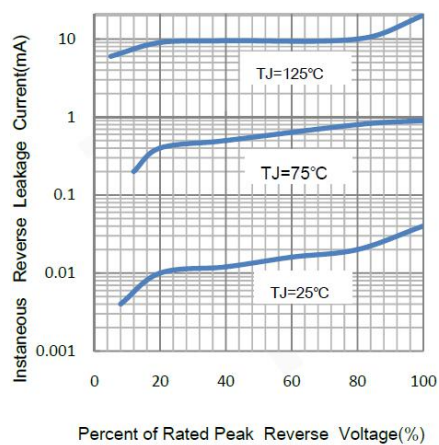
Fig.4 Typical reverse leakage characteristics
